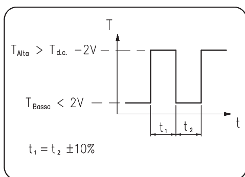
Output signal
