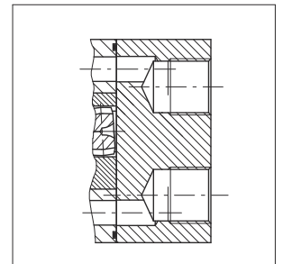
Rear ports configuration.
